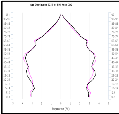
Nene Population age distribution
